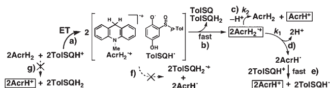
Scheme 1. Mechanism of reduction of TolSQH + by AcrH 2 .
